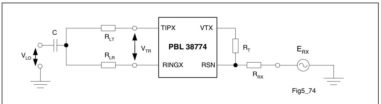
Figure 5 Metallic to Longitudinal, B_{\text{MLE}} and Four-Wire to Longitudinal Balance, B_{\text{FLE}}
