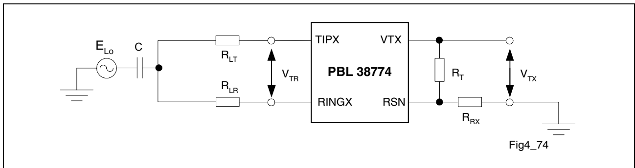
Figure 4 Longitudinal to Metallic, B_{\text{LME}} and Longitudinal to Four-Wire, B_{\text{LFE}} Balance
