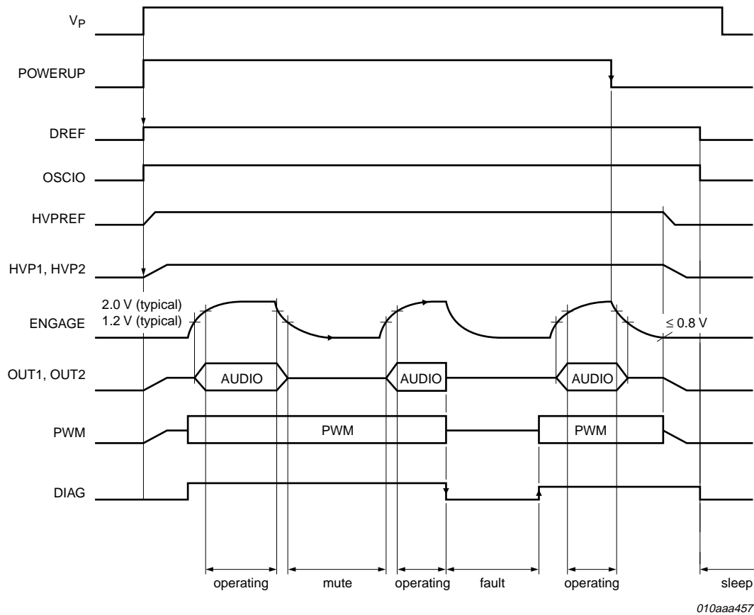
Fig 3. Start-up sequence
