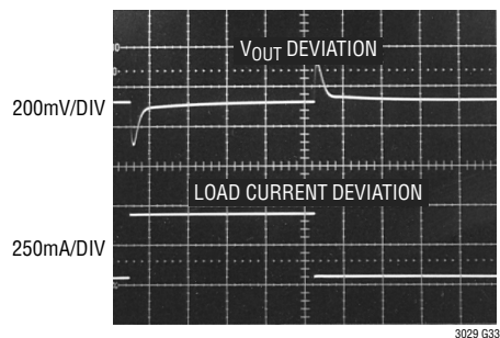
Transient Response, C_{BYP} = 0\text{pF}
