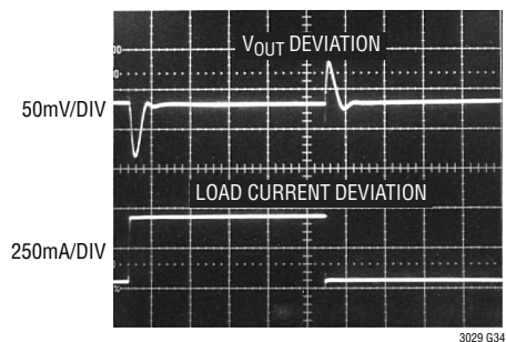
Transient Response, C_{BYP} = 0.01\mu\text{F}
