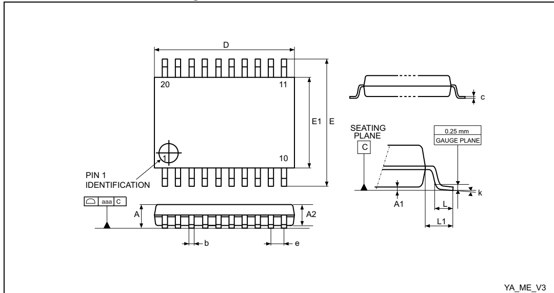
Figure 31. TSSOP20 – Outline
