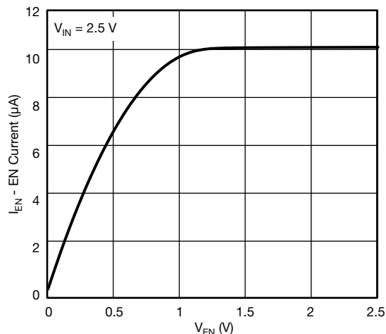
Figure 13 - I_{EN} vs. V_{EN}
