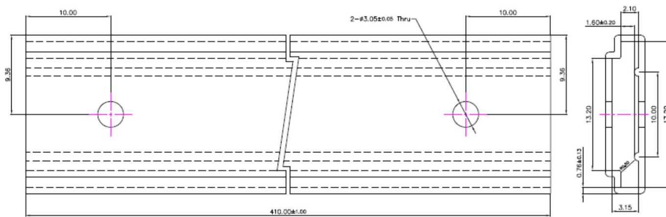
Figure 9. Package ray dimension for LUXEON CoB LHCI – xxxx - I203.
