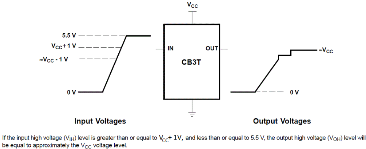
Figure 1. Typical DC Voltage-Translation Characteristics
