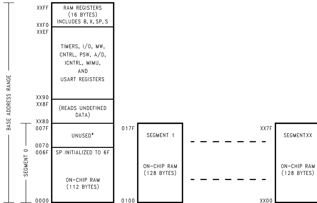
Figure 5-1. RAM Organization
