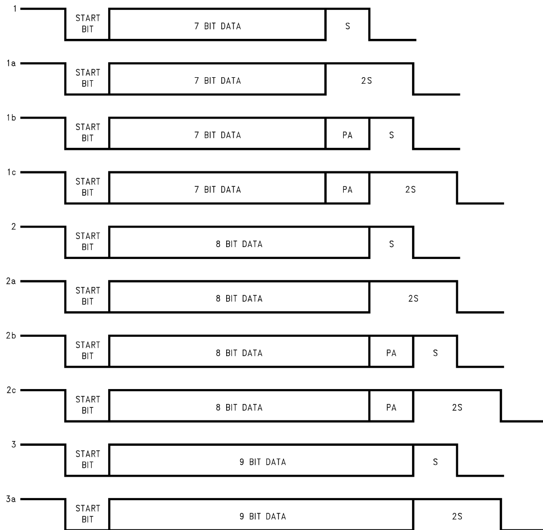
Figure 5-17. Framing Formats
