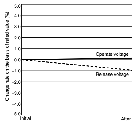
Vibration Resistance
