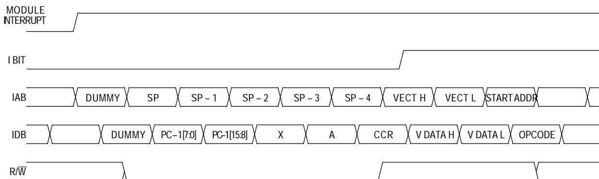
Figure 8. Interrupt Entry
