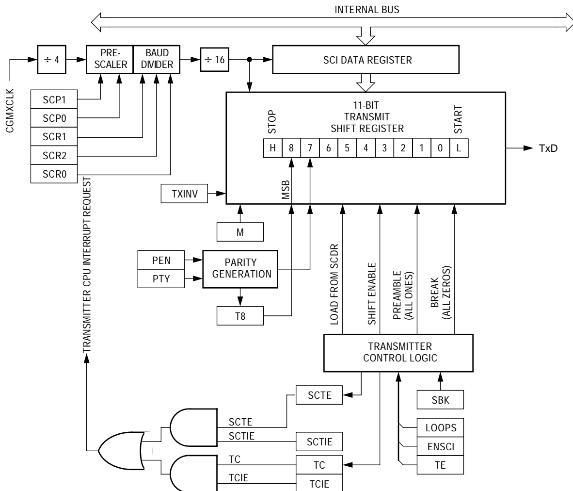
Figure 4. SCI Transmitter
