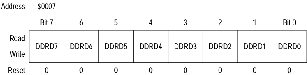
Figure 12. Data Direction Register D (DDRD)
