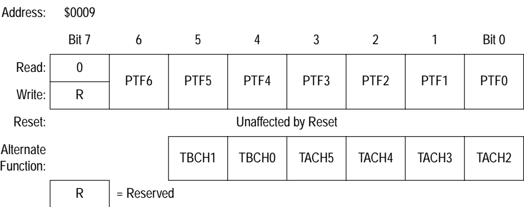
Figure 17. Port F Data Register (PTF)
