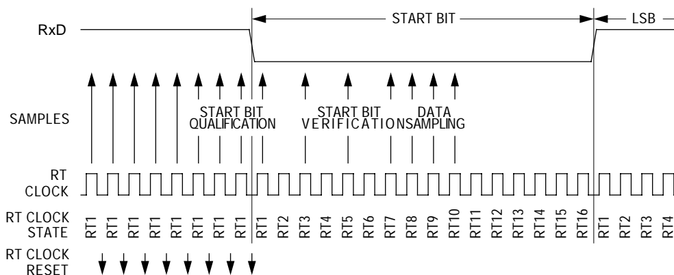
Figure 8. Receiver Data Sampling
