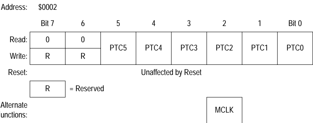
Figure 8. Port C Data Register (PTC)
