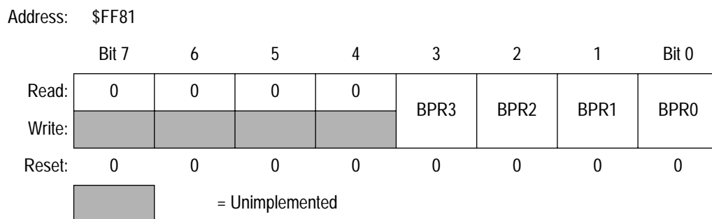
Figure 3. FLASH-2 Block Protect Register (FLBPR2)
