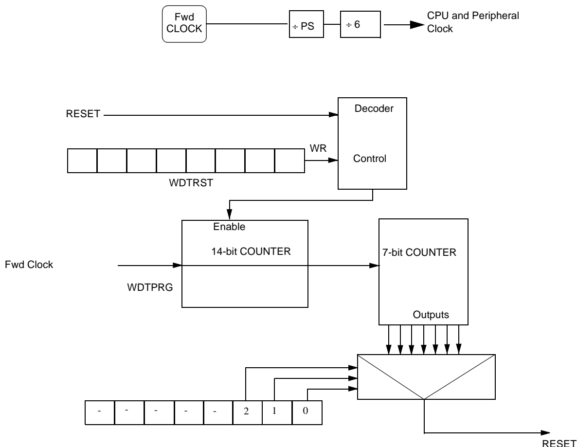
Figure 42. Watchdog Timer
