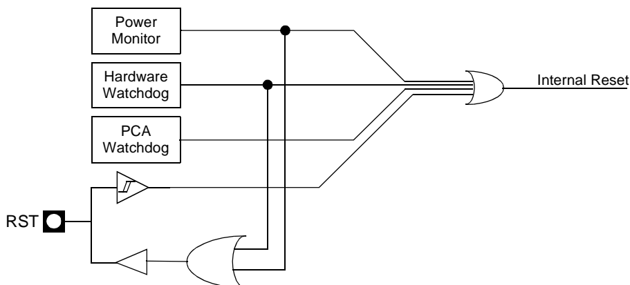
Figure 16. Reset Schematic
