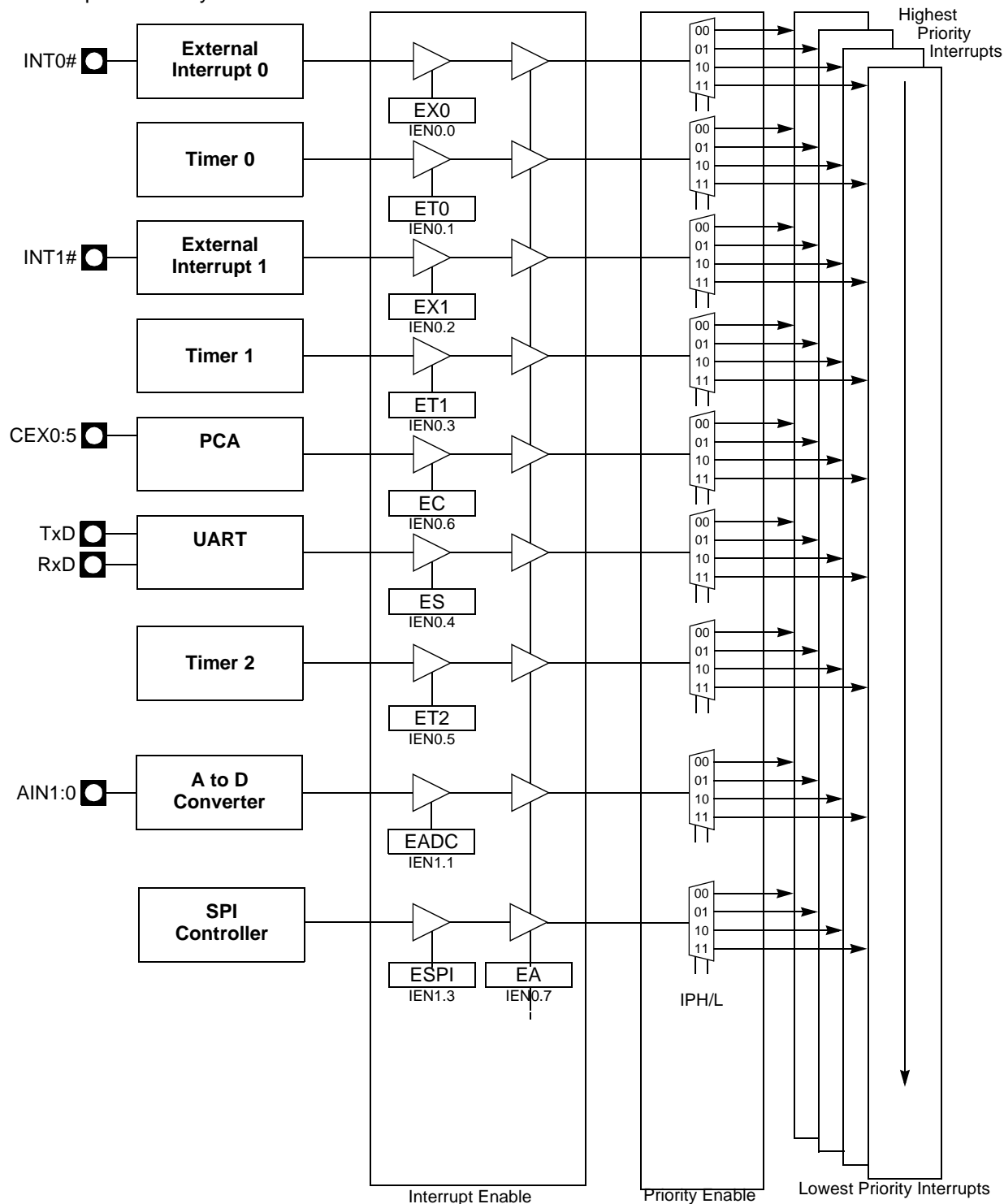
Figure 63. Interrupt Control System
