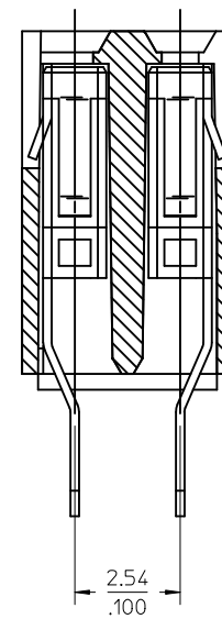
SECTION C-C
