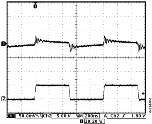
Figure 24. Digital Feedthrough
