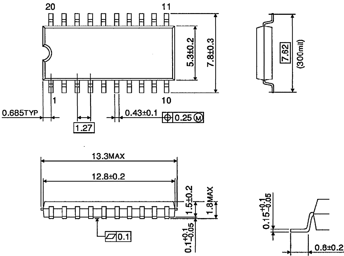
OUTLINE DRAWING SOP20-P-300-1.27
