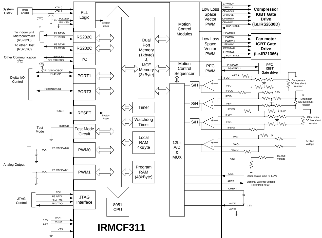
Figure 5. Application Connection of IRMCF311
