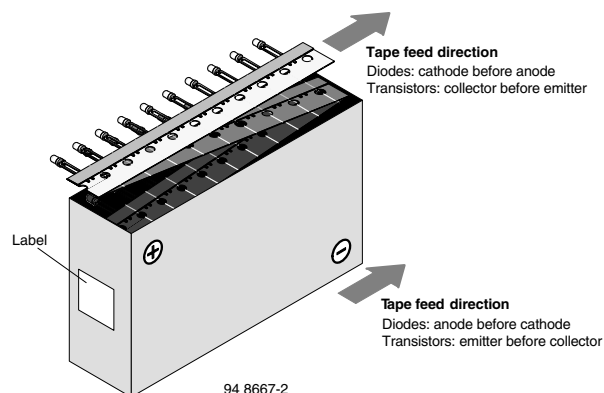
Figure 26. Tape Direction
