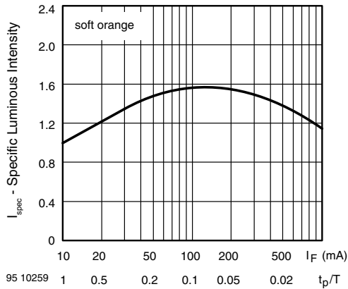
Figure 13. Rel. Lumin. Intensity vs. Forw. Current/Duty Cycle
