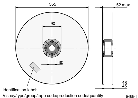
Figure 24. Reel Dimensions
