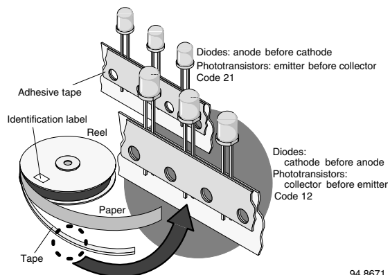
Figure 25. LED in Tape
