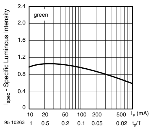
Figure 23. Specific Luminous Intensity vs. Forward Current
