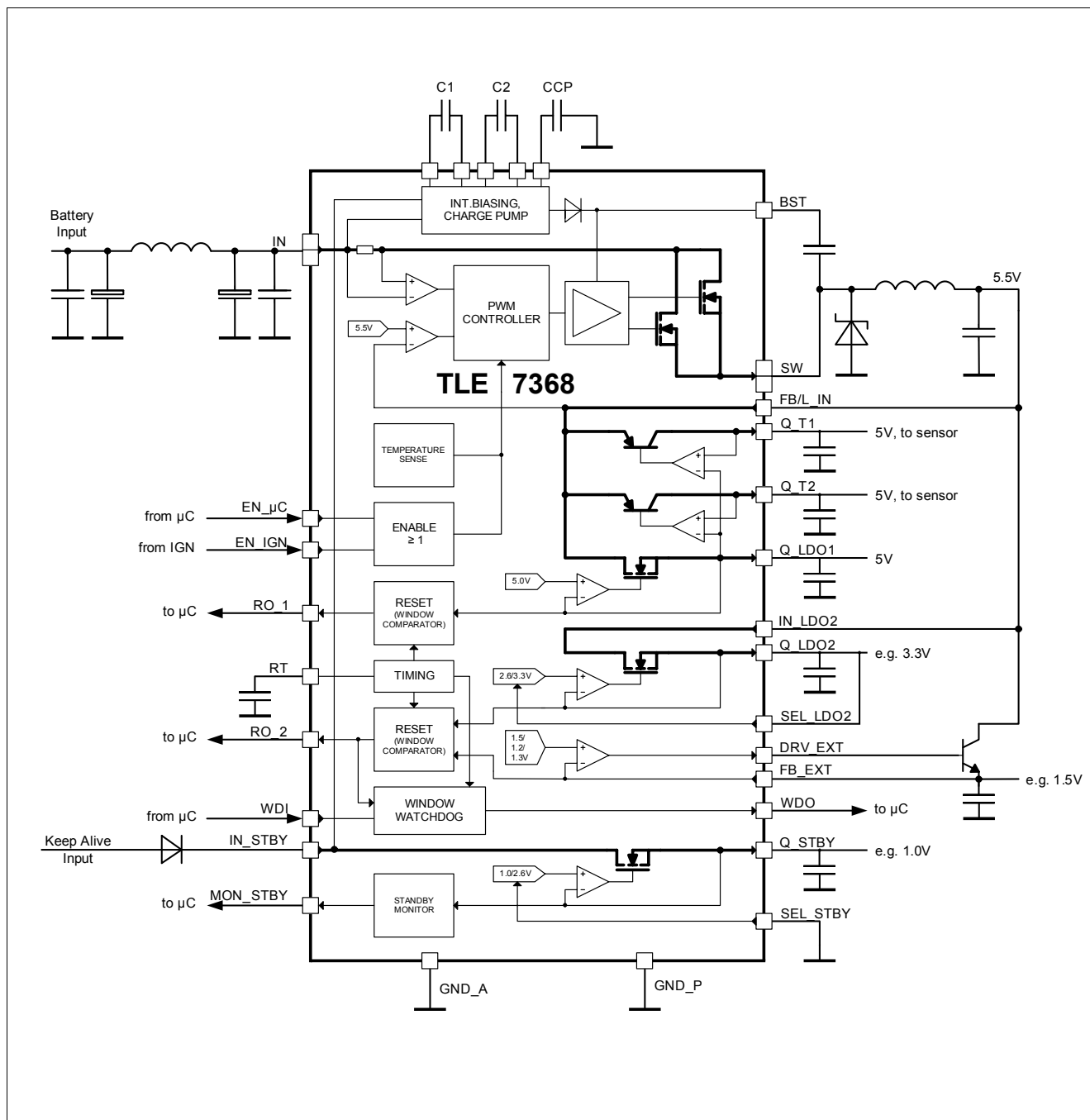
Figure 10 Application Diagram, Example
