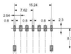
Mounting Dimensions (Top View) Tolerance: \pm 0.1 mm
