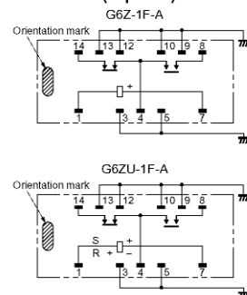
Terminal Arrangement/Internal Connections (Top View)
