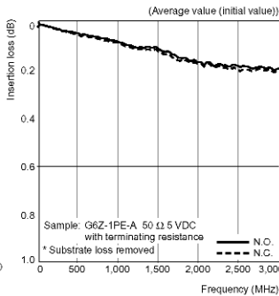
High-frequency Characteristics at 50 \Omega (Insertion Loss)
