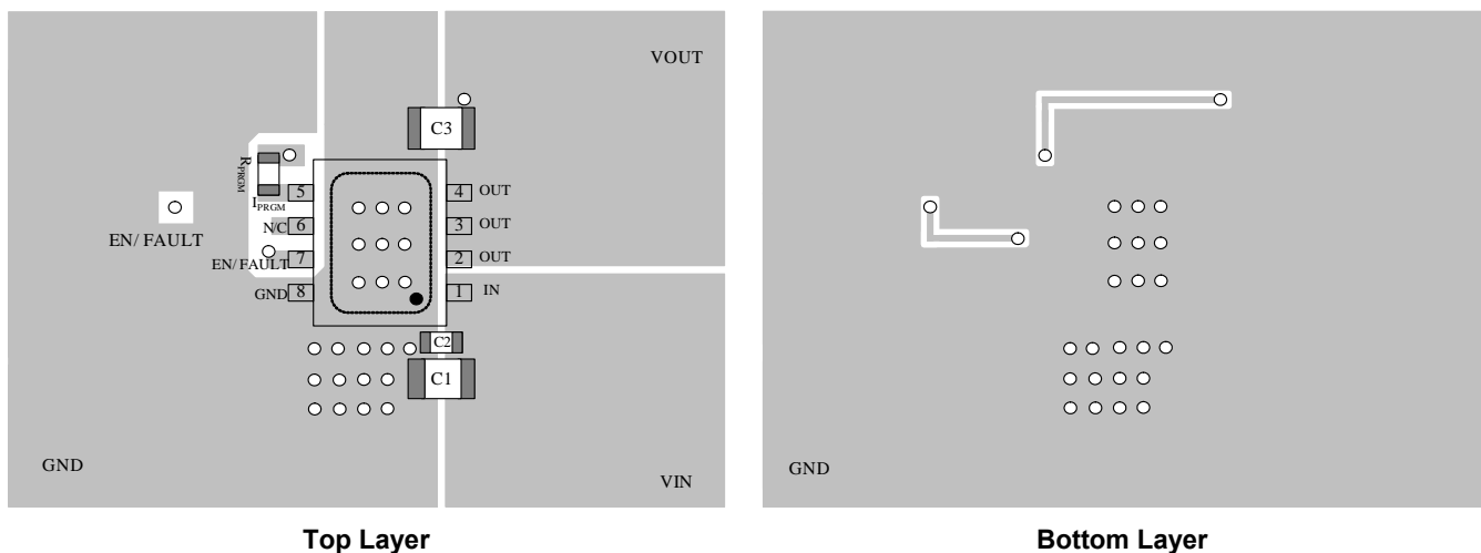
Figure 2—PCB Layout
