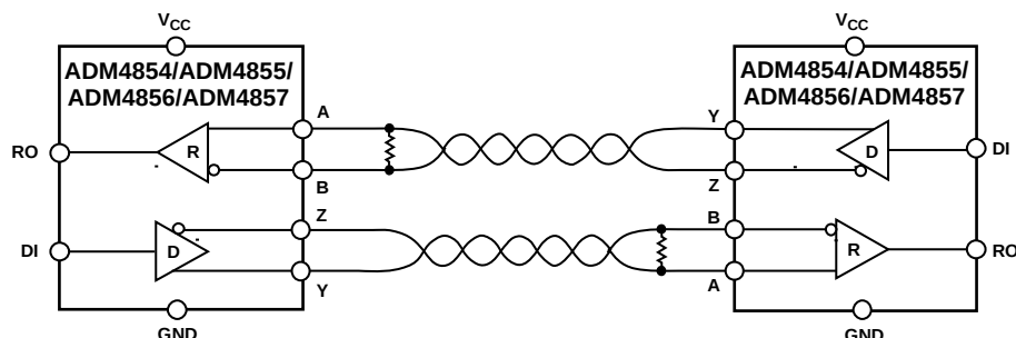
Figure 30. Typical Full Duplex Point-to-Point RS-485 Network Topology
