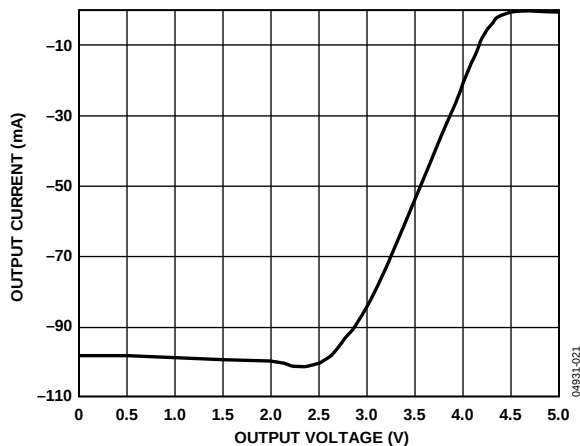
Figure 14. Output Current vs. Driver Output High Voltage
