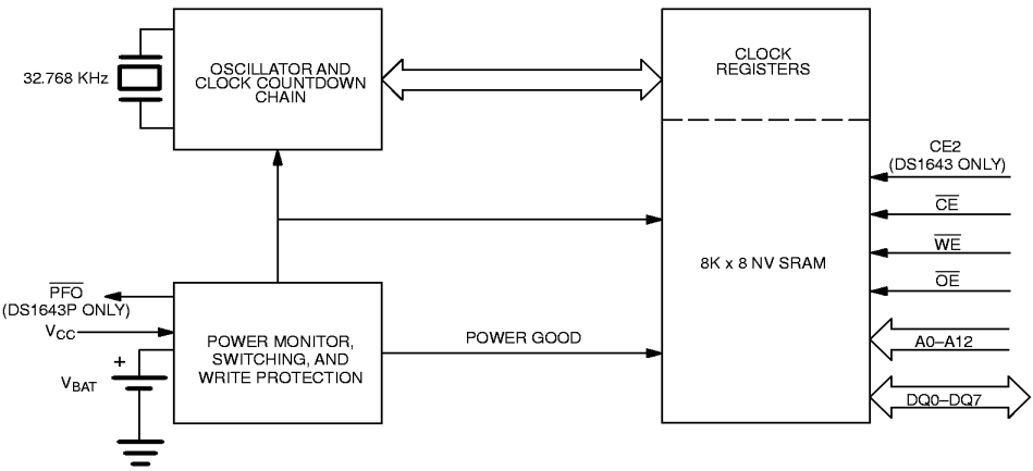
BLOCK DIAGRAM DS1643 Figure 1
