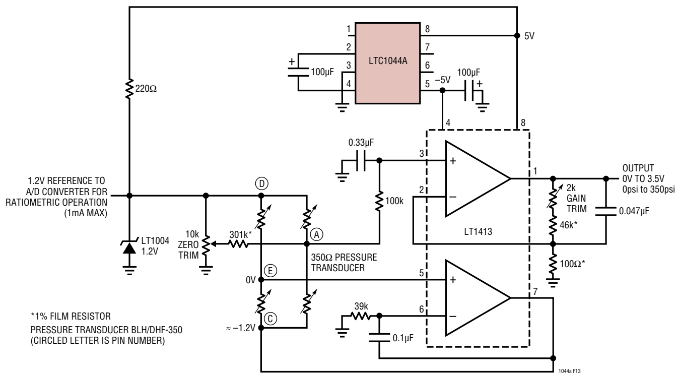
Single 5V Strain Gauge Bridge Signal Conditioner
