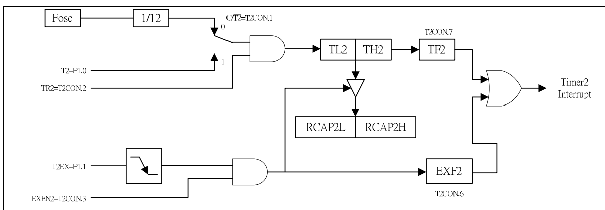
Figure 14-4 16-Bit Capture Mode
