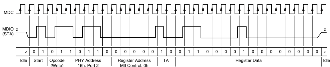
Write Operation
