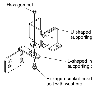
<Side mounting>
