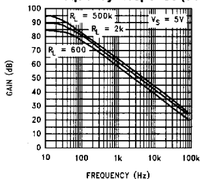
Open Loop Frequency Response (5V)
