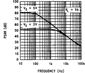
Negative PSRR vs Frequency
