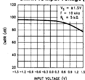
CMRR vs Input Voltage (3V)
