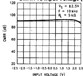
CMRR vs Input Voltage (5V)
