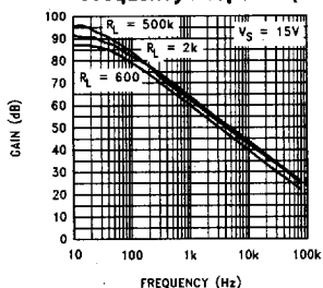
Open Loop Frequency Response (15V)
