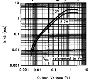
Sinking Current vs Output Voltage (2.7V)
