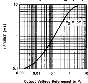
Sourcing Current vs Output Voltage (3V)
