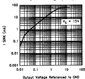
Sinking Current vs Output Voltage (15V)
