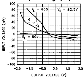
Input Voltage vs Output Voltage (5V)
