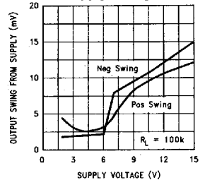
Output Voltage Swing vs Supply Voltage
