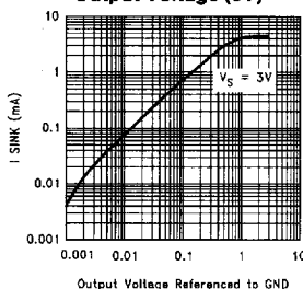
Sinking Current vs Output Voltage (3V)
