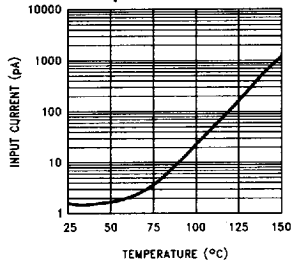
Input Current vs Temperature
