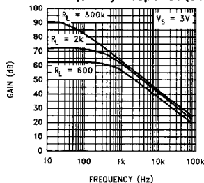
Open Loop Frequency Response (3V)
