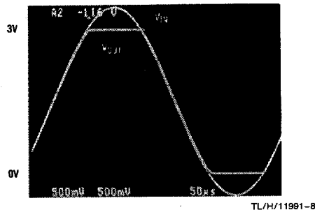
FIGURE 1. An Input Voltage Signal Exceeds the LMC7101 Power Supply Voltages with No Output Phase Inversion
