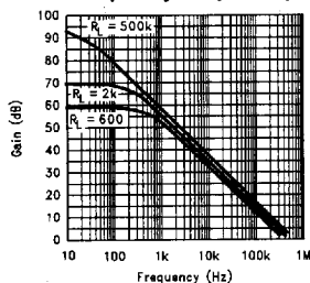
Open Loop Frequency Response (2.7V)
