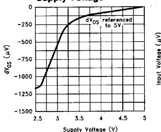
dVos vs Supply Voltage
