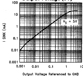
Sinking Current vs Output Voltage (5V)
