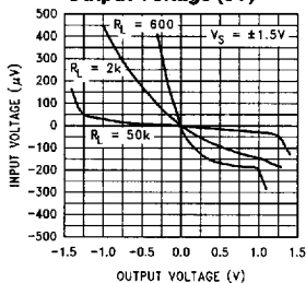
Input Voltage vs Output Voltage (3V)
