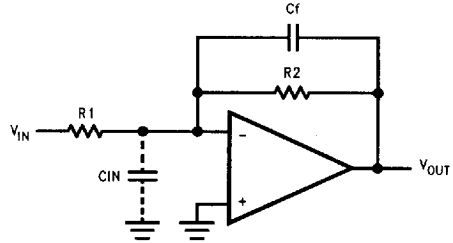
FIGURE 5. Cancelling the Effect of Input Capacitance
