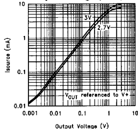
Sourcing Current vs Output Voltage (2.7V)
