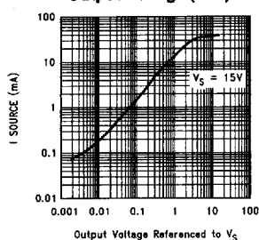
Sourcing Current vs Output Voltage (15V)
