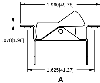
TAPPED HOLE Standard with A Bracket
