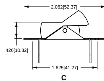
CLEARANCE HOLE Standard with C Bracket
