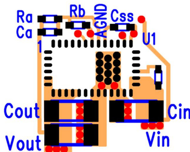
Figure 7: Top PCB Layer Critical Components and Copper for Minimum Footprint
