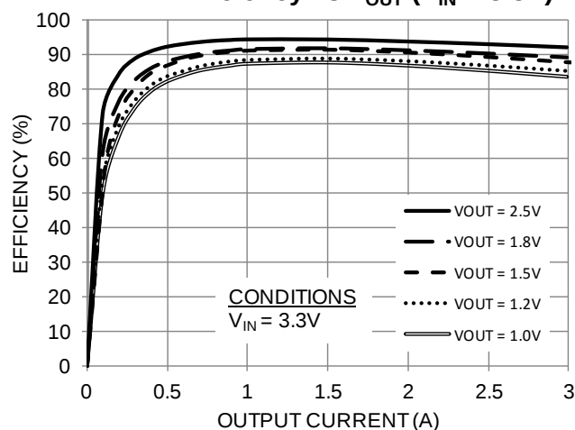
PWM Efficiency vs. I_{OUT} ( V_{IN} = 3.3V )
