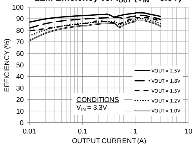
LLM Efficiency vs. I_{OUT} ( V_{IN} = 3.3V )
