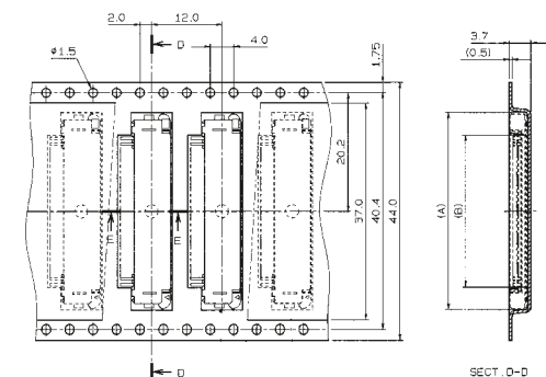
SECT. D-D
