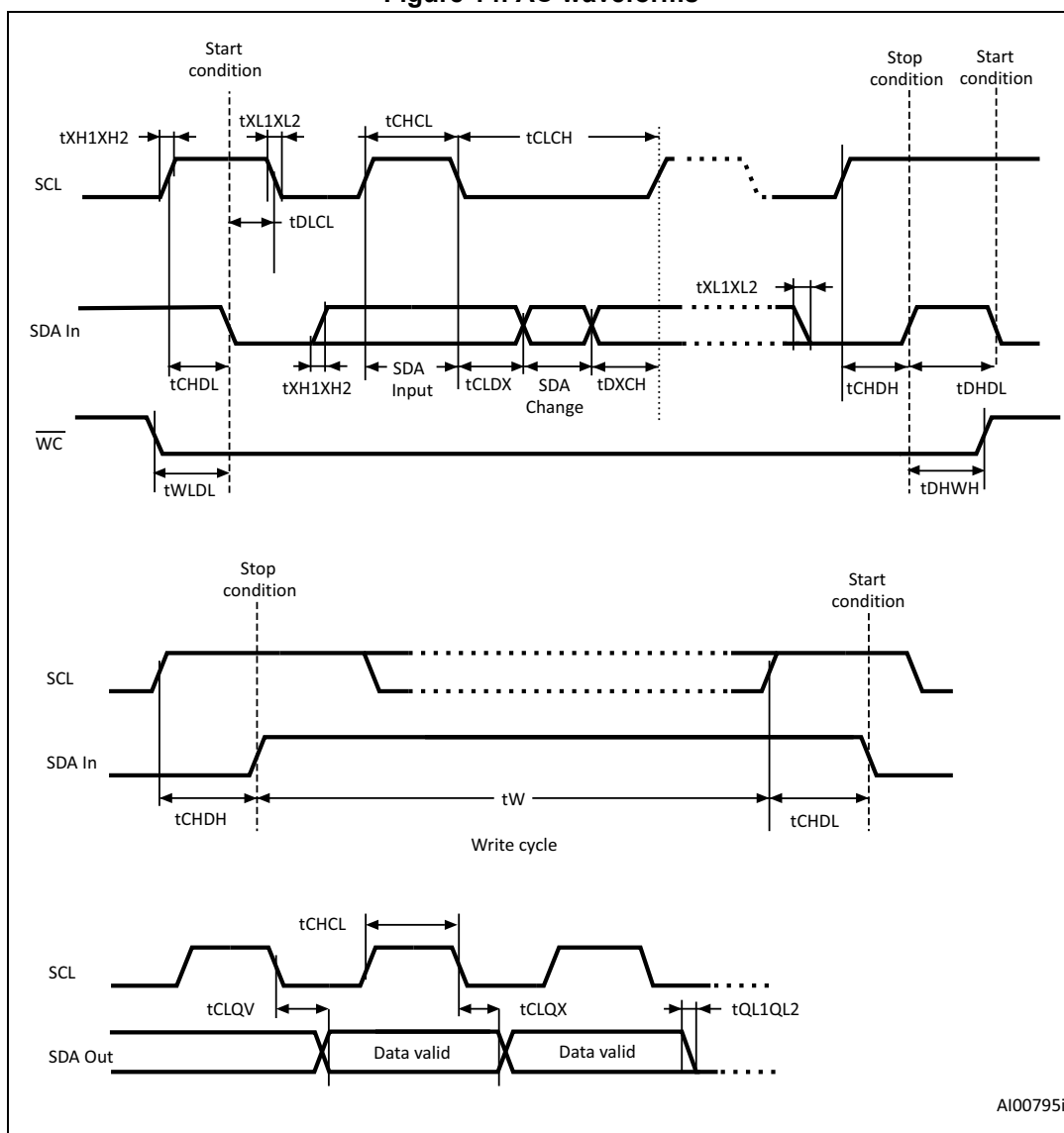
Figure 14. AC waveforms
