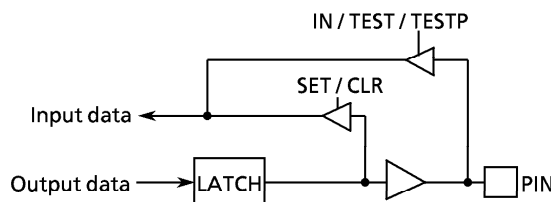
Figure 3-2. Port R3
