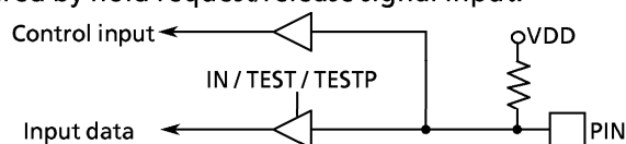
Figure 3-1. Port K0
