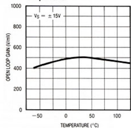
Open-Loop Gain vs Temperature
