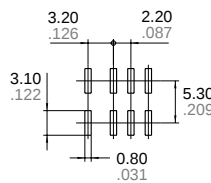
Suggested mounting pad
