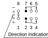
Single side stable (Deenergized condition)
