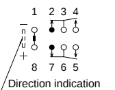
1 coil latching (Reset condition)
