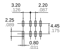
Suggested mounting pad
