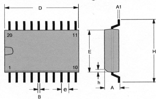
HMC1002—Package Outline
