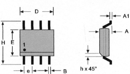
HMC1021S—8-Pin SOIC
