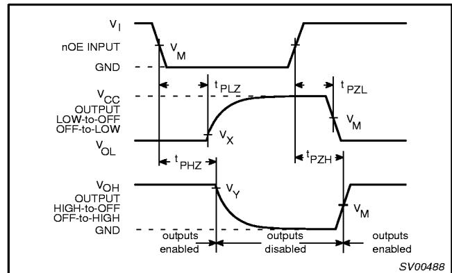
Figure 2. 3-state enable and disable times.
