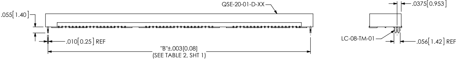
FIG 2 -LC: LOCKING CLIP OPTION (QSE-060-01-XXX-D-LC SHOWN) (DIFFERENT AS SHOWN, OTHERWISE SAME AS FIG 1)
