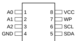
8-lead SOIC
