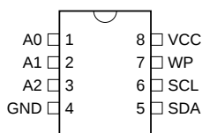
8-lead PDIP
