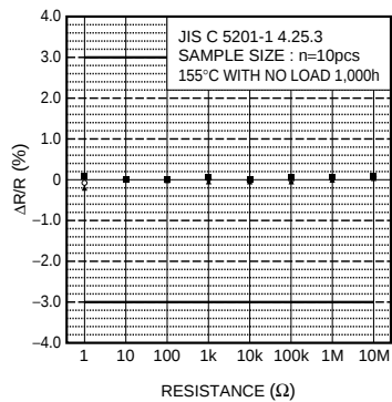
Fig.12 Endurance
