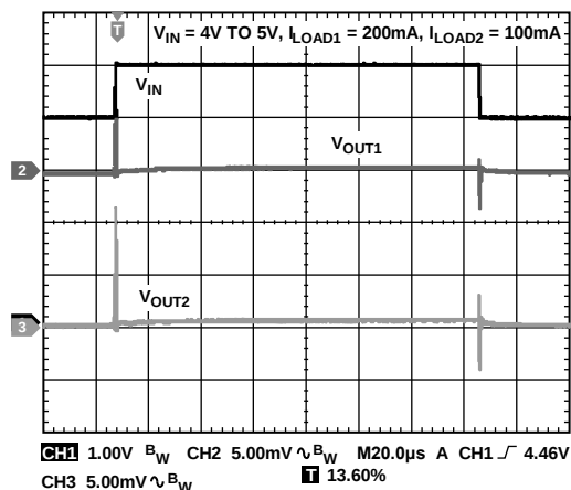
Figure 25. Line Transient Response, V_{IN} = 4\text{ V to } 5\text{ V} , I_{LOAD1} = 200\text{ mA} , I_{LOAD2} = 100\text{ mA} CH1 = V_{IN} , CH2 = V_{OUT1} , CH3 = V_{OUT2}
