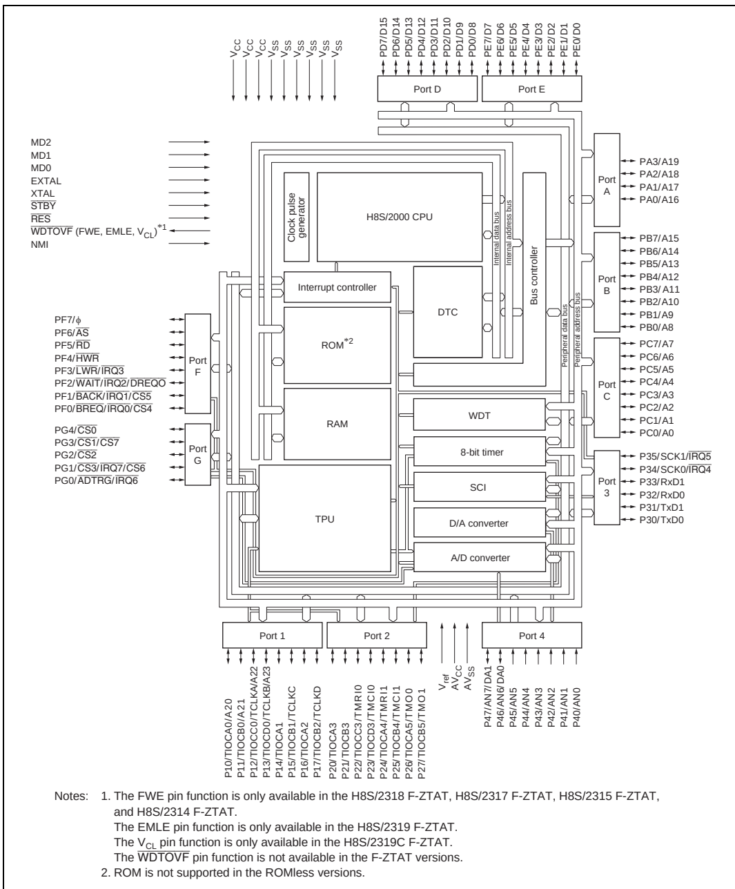
Figure 1.1 Block Diagram
