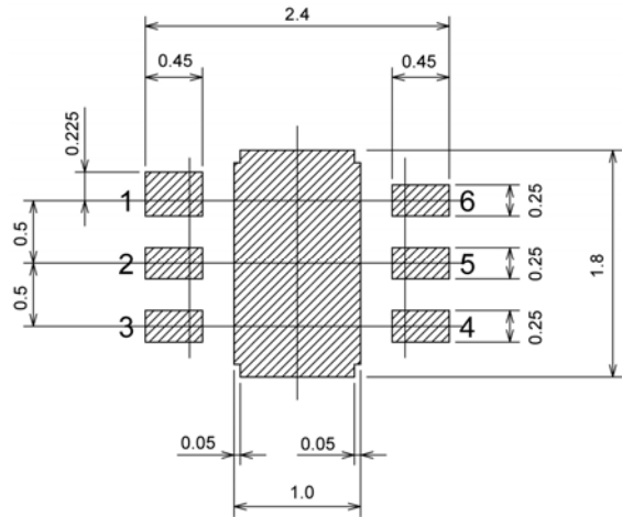
●USP-6C Reference Pattern Layout
