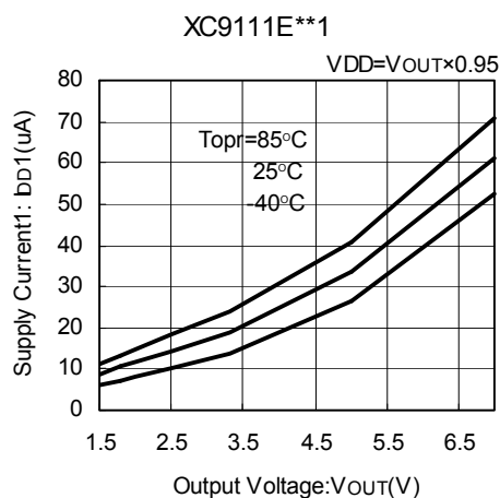
(4) Supply Current 1 vs. Output Voltage
