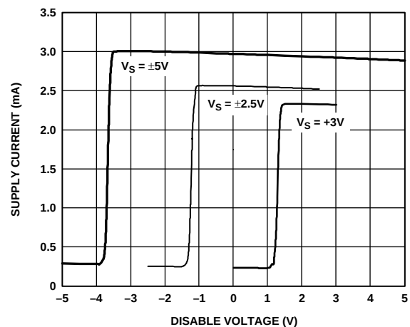
Figure 26. Supply Current vs. \overline{POWER\ DOWN} Pin Voltage
