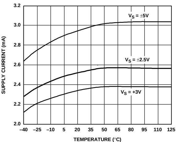
Figure 30. Supply Current vs. Temperature for Various Supplies
