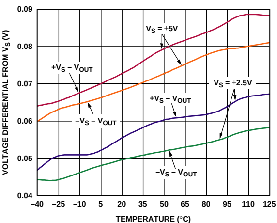
Figure 29. Output Saturation vs. Temperature for Various Supplies
