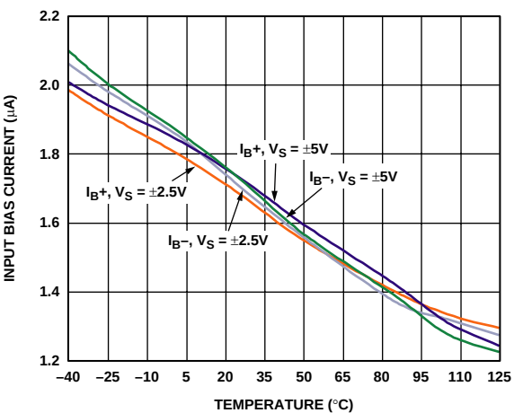
Figure 28. Input Bias Current vs. Temperature for Various Supplies
