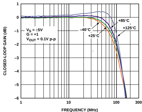
Figure 8. Small Signal Frequency Response for Various Temperatures
