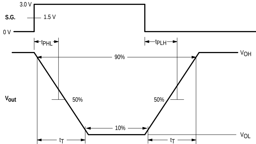
Figure 1. Timing Diagram
