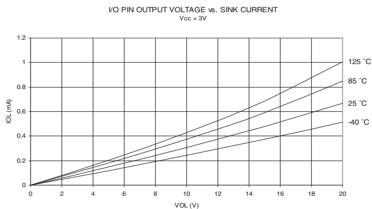
Figure 28-12. Output Low Voltage vs. Output Low Current ( V_{CC} = 3.0V )
