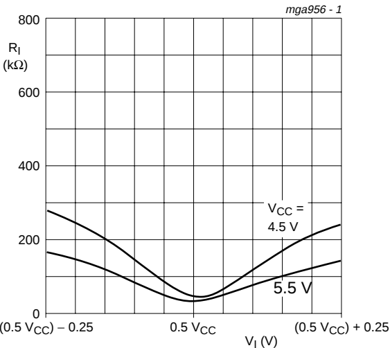
Fig 15. Input resistance at SIG_IN; COMP_IN with \Delta V_I = 0.5\text{ V} at self-bias point
