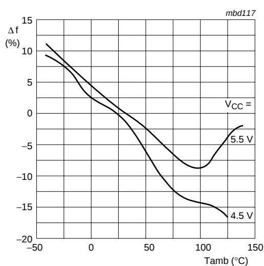
Fig 21. Frequency stability of the VCO as a function of ambient temperature with supply voltage as a parameter
