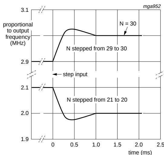
Fig 36. Frequency compared to the time response
