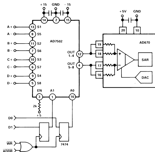
Figure 16. Multiplexed Analog Inputs to AD670
