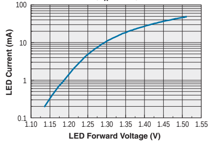
CPC1302 LED Current ( I_F ) vs. LED Forward Voltage ( V_F ) ( T_A = 25^\circ\text{C} )
