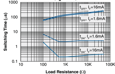
CPC1302 Switching Time vs. Load Resistance ( T_A = 25^\circ\text{C} )
