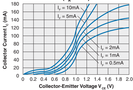
CPC1302 Collector Current vs. Collector-Emitter Voltage ( T_A = 25^\circ\text{C} )
