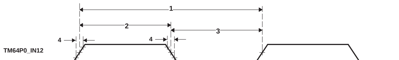
Figure 6-80. Timer Timing
