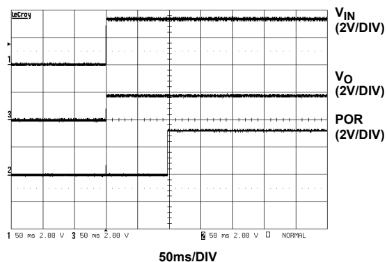
FIGURE 8. START-UP 2
