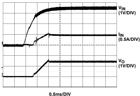
FIGURE 7. START-UP 1
