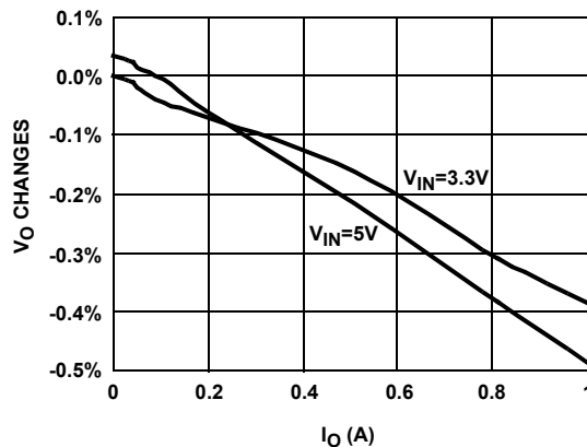
FIGURE 4. LOAD REGULATIONS
