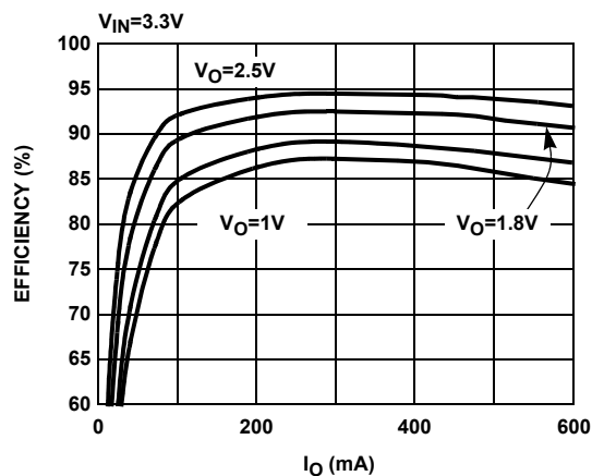
FIGURE 2. EFFICIENCY
