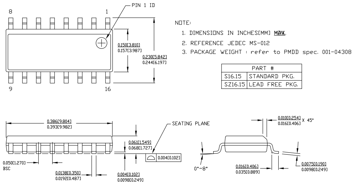
Figure 15. 16-pin SOIC (150 Mils) Package Outline, 51-85068
